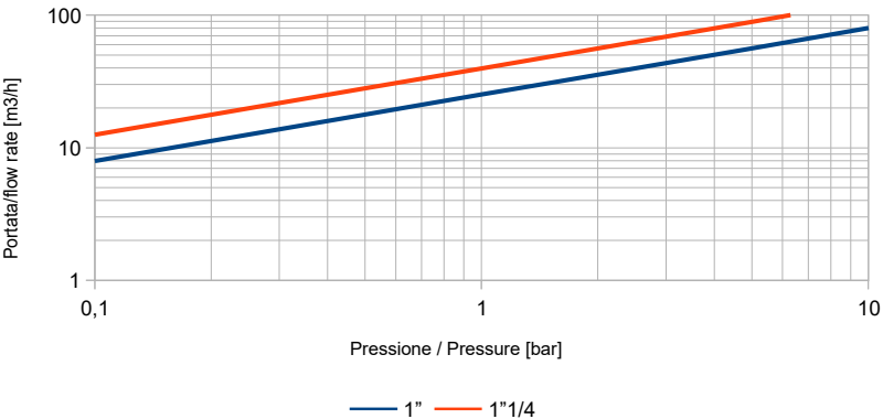
Filtro Acqua - Water Strainer Art. 7009 "AMALFI"
