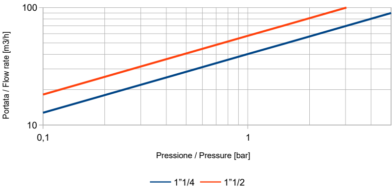
Filtro Acqua - Water Strainer Art. 0008 "VENEZIA COMPACT"
