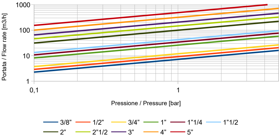
Filtro Acqua - Water Strainer Art. 0005 / 2005 / 7005 / 0105 / 2105 / 7105 "GENOVA"
