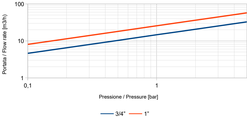
Filtro Acqua - Water Strainer Art. 2009 "AMALFI"
